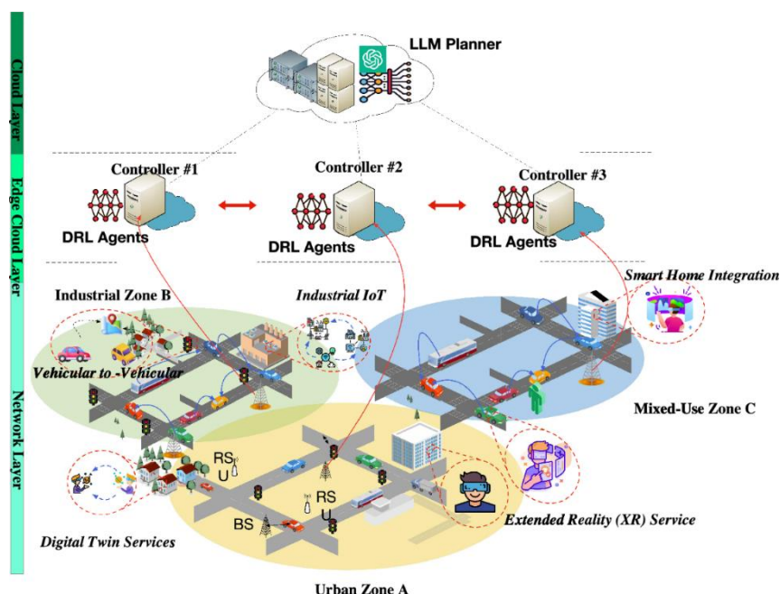
FIG1: Cloud-Native Enterprise Automation through Intelligent Workflow Orchestration
