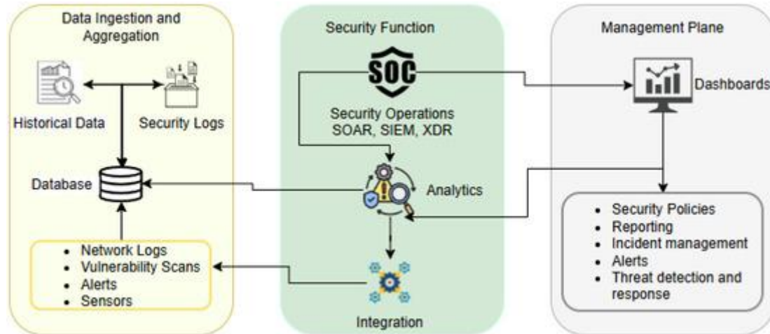
Fig.1. Cloud Security Automation through Symmetry: Threat Detection and Response
