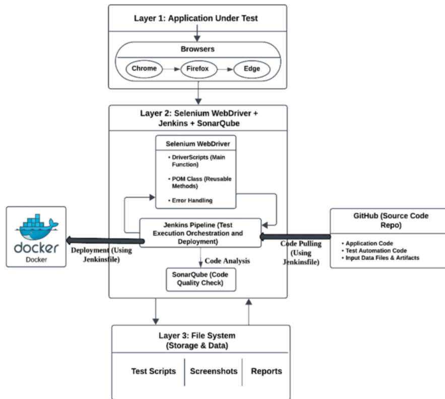
Fig.1. Enhancing software quality of CI/CD pipeline through continuous testing: a DevOps-driven maintainable hybrid automation testing framework
