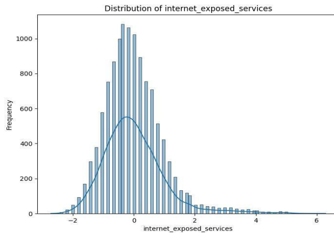
Fig.1. Distribution of internet_exposed_services: right-skewed with positive outliers indicating elevated attack surface exposure.
