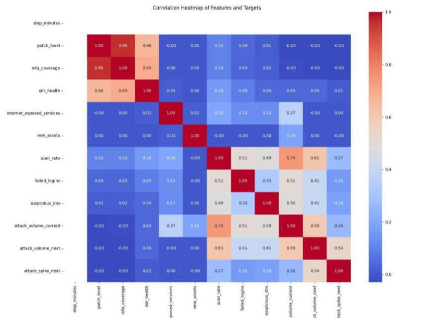
Fig.3. Correlation heatmap of all features and target variables. Strong interdependencies are observed between security posture metrics and between scan-rate-based features and attack volume targets.
