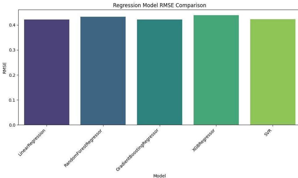
Fig.7. Regression Model RMSE Comparison. All models converge within a narrow RMSE band (0.422–0.439), suggesting saturation of predictive capability under standard supervised learning with the current feature set.
