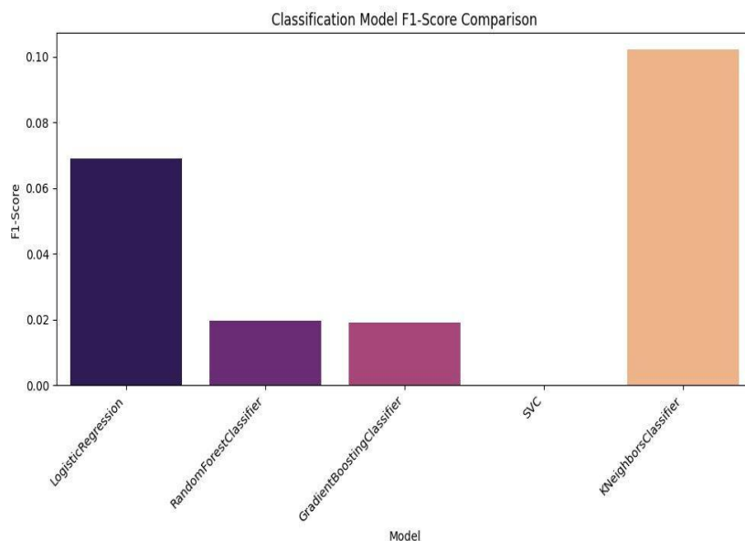
Fig.5. Classification Model F1-Score Comparison. KNN achieves the highest F1-Score (0.102), followed by Logistic Regression (0.069), reflecting superior minority-class detection capability under severe class imbalance.
