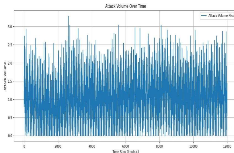
Fig.4. Attack volume over time across 11,999 monitoring steps, showing high-frequency volatility with recurrent spike events indicative of coordinated attack bursts
