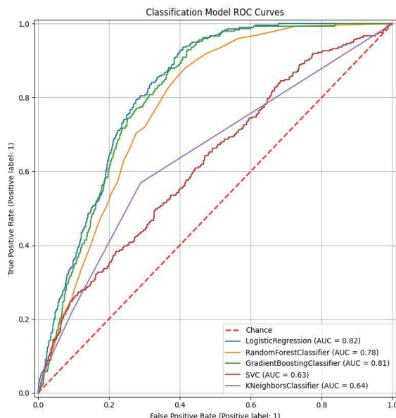
Fig.6. ROC Curves for all classification models. Logistic Regression (AUC=0.82) and Gradient Boosting (AUC=0.81) demonstrate the strongest discriminative power, while SVC (AUC=0.63) approaches the random baseline.
