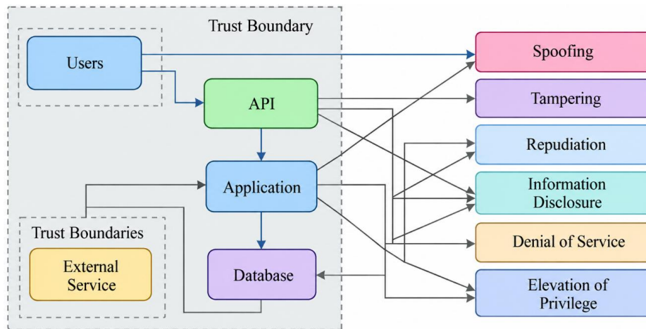
Figure 3- Architecture-Aware STRIDE Threat Mapping
