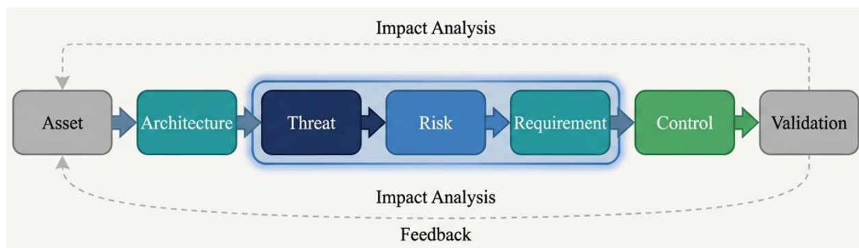
Figure 4- Security Traceability Chain
