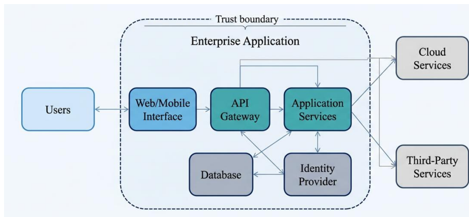
Figure 2- Enterprise Application Security Context Model
