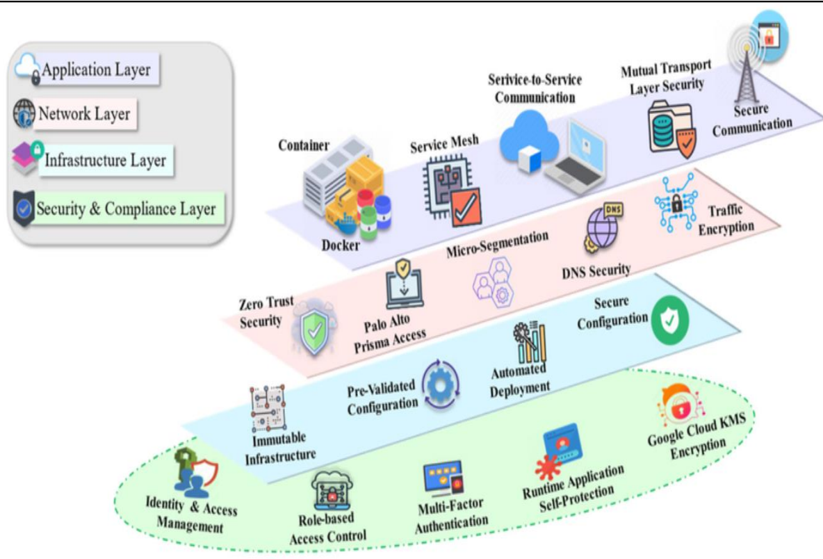
Figure: Architecture of an AI-Enabled Secure and Compliant Enterprise Data Platform for Cross-Cloud Analytics, Cybersecurity, and Intelligent Automation
